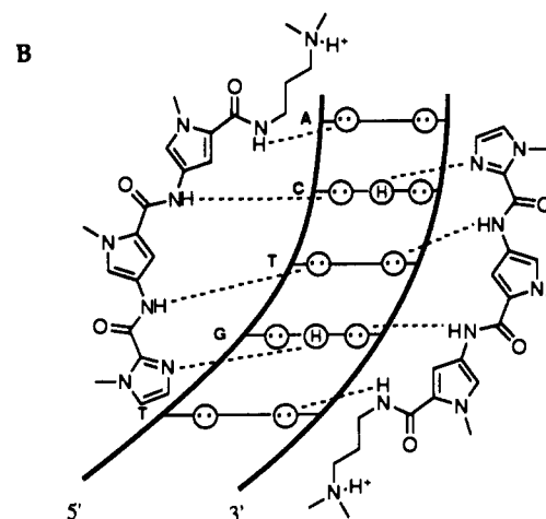
Figure 3. Homodimeric binding models for the complexes formed between (A) 2-PyN and (B) 2-ImN with the 5'-TGCTA-3' sequence. 11 Circles with dots represent lone pairs of N3 of purines and O2 of pyrimidines. Circles containing an H represent the N2 hydrogen of guanine. Putative hydrogen bonds are illustrated by dashed lines.
